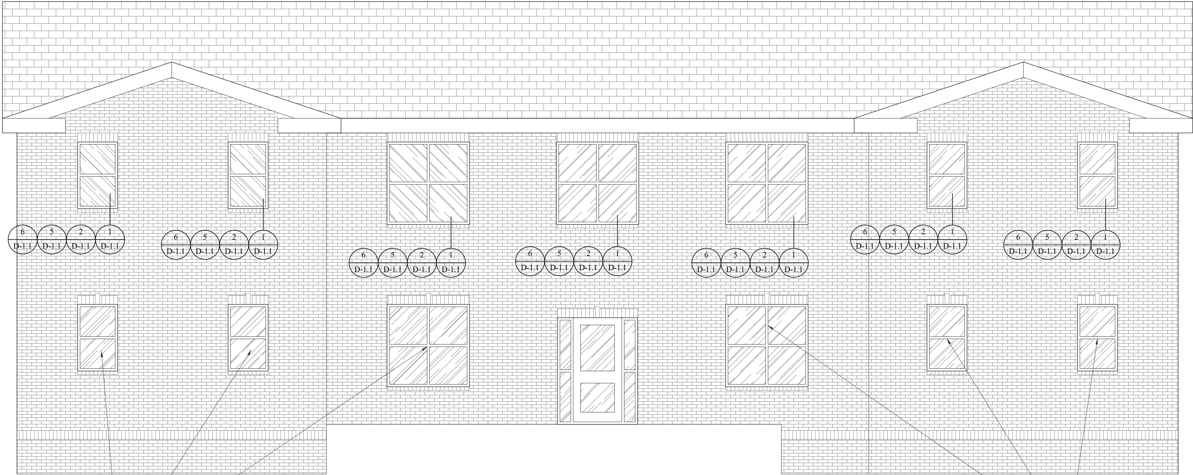
1 SOUTH FACING ELEVATION PLAN R-1.1 1/4" = 1'
